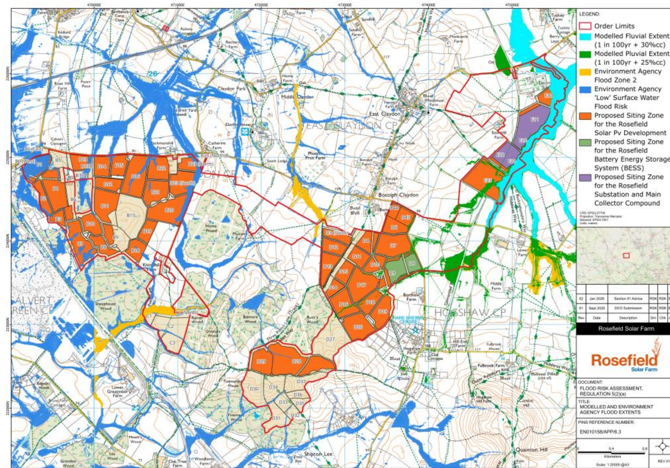
Figure 3.7: Credible Maximum Flood Extents
